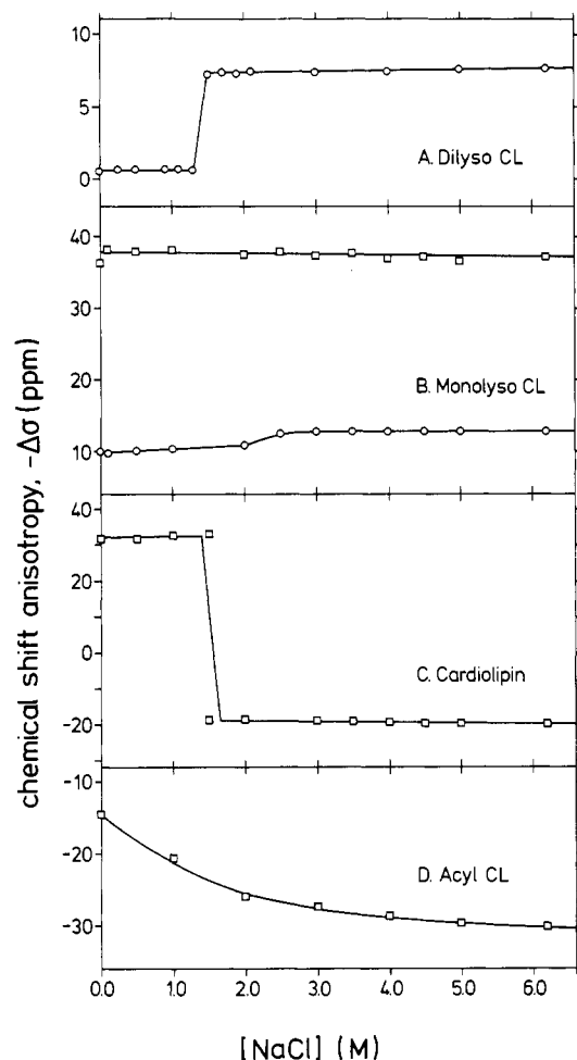
FIGURE 3: ^{31}\text{P} chemical shift anisotropy, \Delta\sigma , at 20^\circ\text{C} as a function of NaCl concentration for (A) dilyso-cardiolipin, (B) monolyso-cardiolipin, (C) cardiolipin, and (D) acylcardiolipin.
