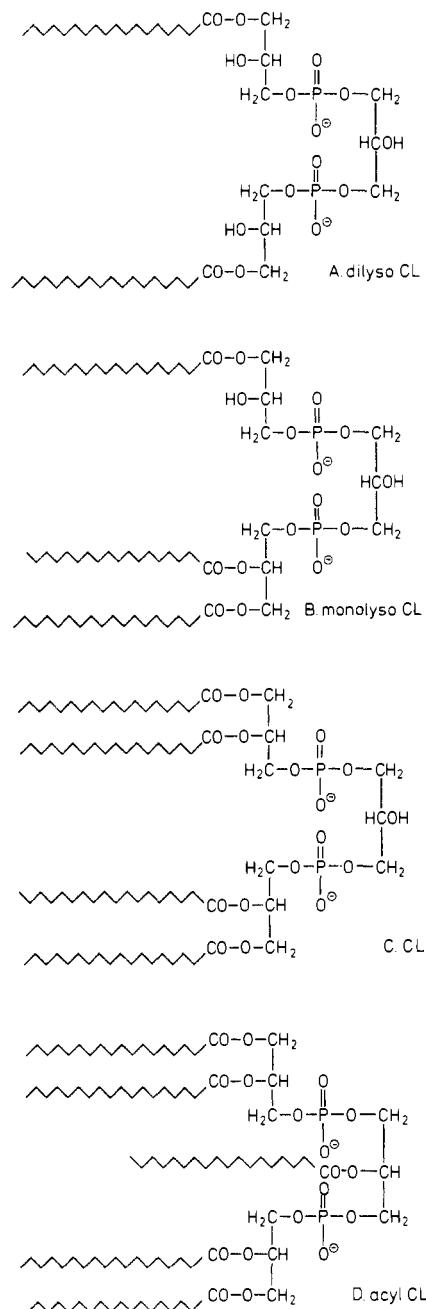
FIGURE 1: Structures of cardiolipin derivatives: (A) dilyso-CL; (B) monolyso-CL; (C) CL; (D) acyl-CL. The acyl chains are indicated schematically. For beef heart CL analogues, the phosphatidyl chains are 87% linoleoyl. For acyl-CL, the 2-acyl chain is oleoyl.
