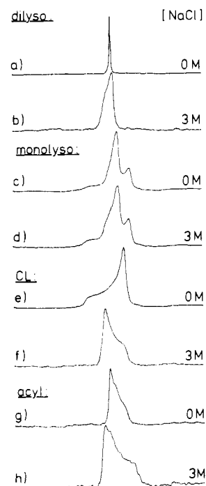
FIGURE 2: Proton dipolar-decoupled 109-MHz ^{31}\text{P} NMR spectra of cardiolipin derivatives dispersed in 0.0 and 3.0 M NaCl at 20 °C: (a) dilyso-CL in 0.0 M NaCl; (b) dilyso-CL in 3.0 M NaCl; (c) monolyso-CL in 0.0 M NaCl; (d) monolyso-CL in 3.0 M NaCl; (e) CL in 0.0 M NaCl; (f) CL in 3.0 M NaCl; (g) acyl-CL in 0.0 M NaCl; (h) acyl-CL in 3.0 M NaCl. Plot width = 16 kHz (146 ppm).
