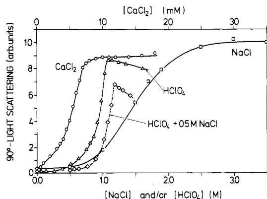
FIGURE 4: 90^\circ light scattering at 460 nm of dilyso-cardiolipin dispersions (1 mg/3 mL) as a function of salt or acid concentration: ( \square ) NaCl; ( \circ ) \text{CaCl}_2 [note 100-fold expansion of (upper) concentration scale]; ( \Delta ) \text{HClO}_4 ; ( \diamond ) \text{HClO}_4 in the presence of 0.5 M NaCl [note that the horizontal scale is the total concentration ( [\text{HClO}_4] + [\text{NaCl}] ) in this case]. Dispersions contained 1 mM EDTA (except for \text{CaCl}_2 ), pH 7.4.
